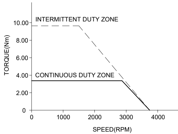
SPEED - TORQUE CURVE
